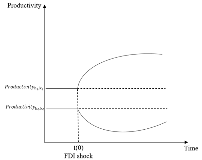
Figure 2: Theoretical shock considering different productivity levels.
